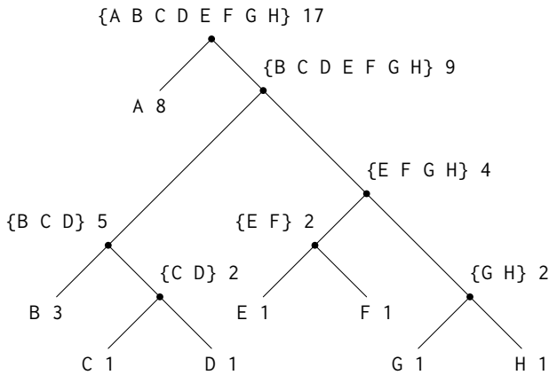
Figure 2.18: A Huffman encoding tree.
