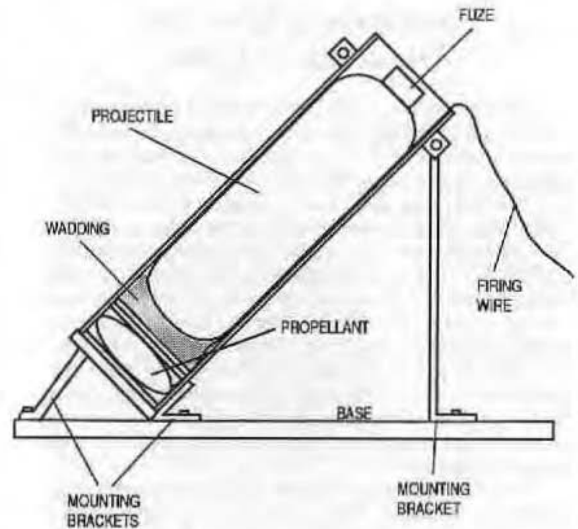
Sectioned view of IRA truck mortar.
