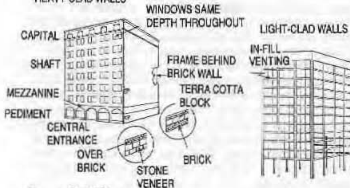
Framed buildings.
