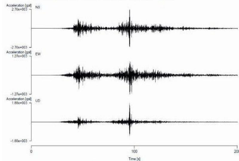
Acceleration recorded at station MYG004 displaying the largest PGA measured (this KNET station is located near Kurihara)
